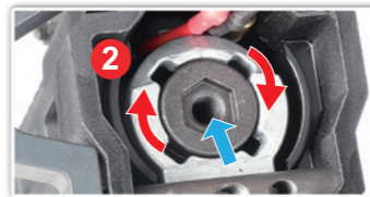
Use 8mm Allen key to depress the spring guide and rotate 45°, carefully and slowly remove the guide.
