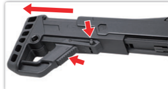
Press and hold the unlock button and stock adjustment button to remove the stock.
