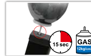
Add gas through the valve at the bottom of the magazine.
