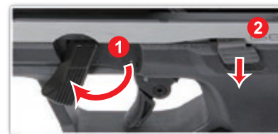
Rotate the take-down lever and press down the slide stop.
