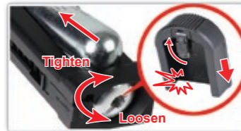
Tab on the rear of the magazine bottom plate then flip out the hex key. Use the hex key to loosen the cartridge tray at the bottom. Install the CO2 cartridge into the magazine and tighten up the tray.
