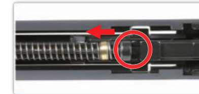
Push forward the recoil spring guide rod and compress the recoil spring.
