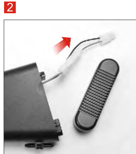
Remove the butt plate and pull out the connector.
